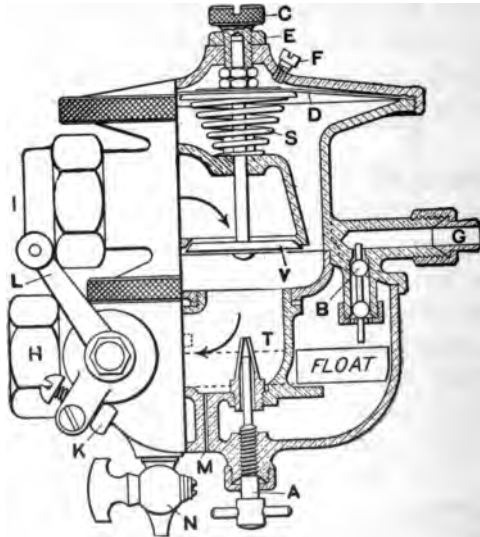
FIG. 163.—The "Kingston" Automatic Float-feed Sprayer.
